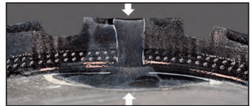
Proper tire repair.
