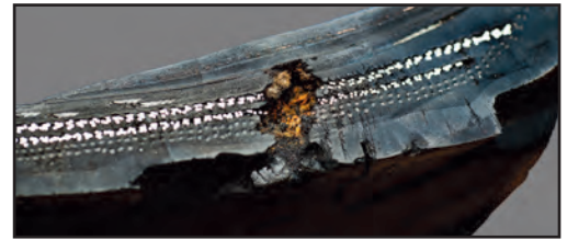
Improper tire repair.
